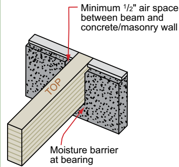
G6 Beam to Concrete / Masonry Wall
