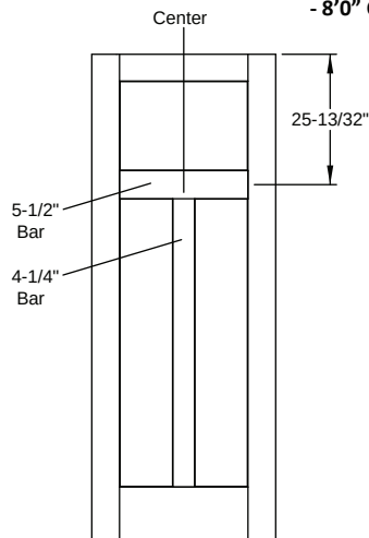
Door Divider - Opaque / SDL - Flush Glazed Classic Craft Shaker American - 8'0" 2 Panel Craftsman Shaker - 8'0" Craftsman 3 Lite
