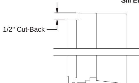
Composite Outswing Sill (Patio Mullion Must Be Used)
