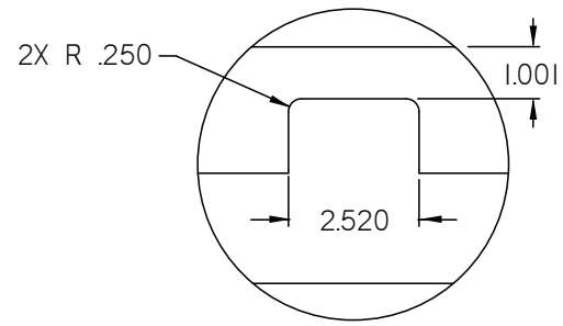
WIDE MULLION
