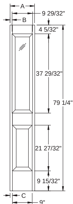
Fiber-Classic/ Smooth-Star/ Steel Panel Dimensions
