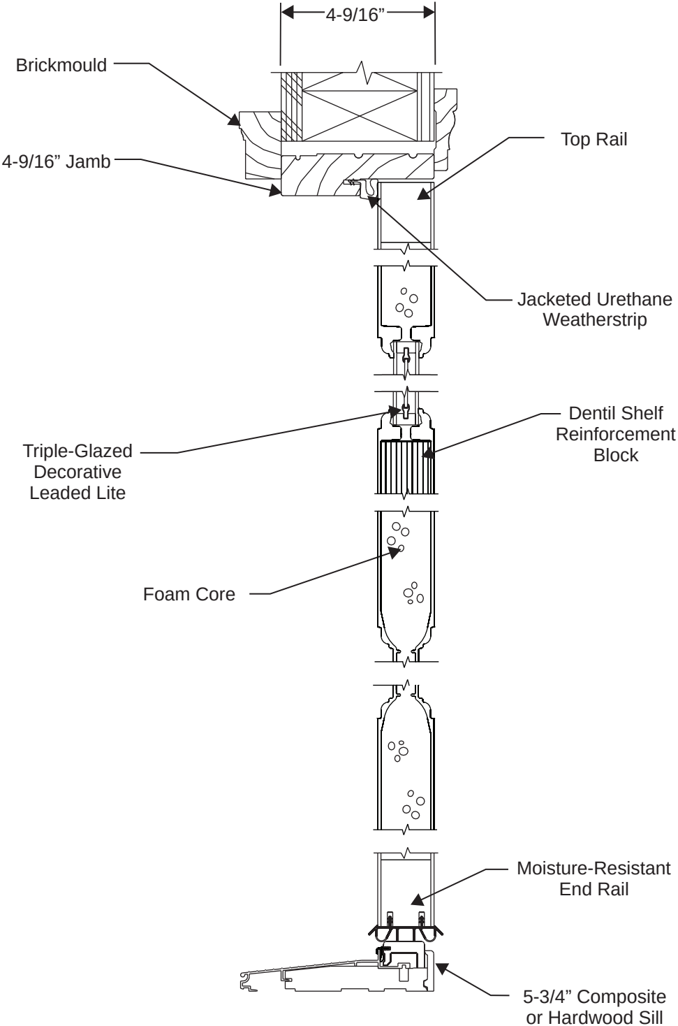
SECTION B-B
