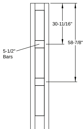
SDL - Flush-Glazed Classic Craft Shaker American - 8'0" Colonial 5 Lite
