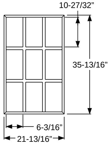
9-Lite PG2236L9
