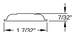
Mull Casing Standard Outswing
