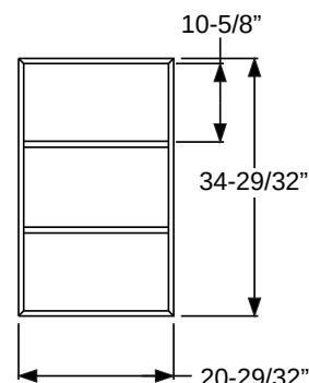
3-Lite (2236)
