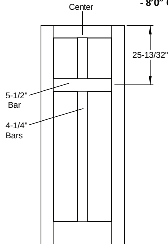
Door Divider - Opaque / SDL - Flush Glazed Classic Craft Shaker American - 8'0" 4 Panel Craftsman Shaker - 8'0" Craftsman 4 Lite
