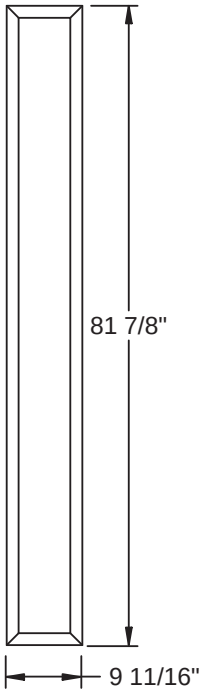
0780H Impact
