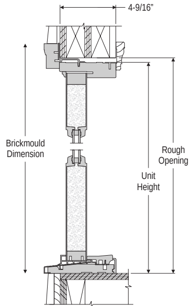
VERTICAL SECTION OUTSWING - FIXED
