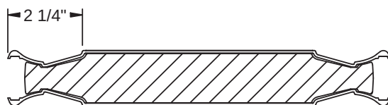
Frame Profile
