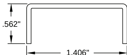
Composite Jamb Patio Screen Track Cover
