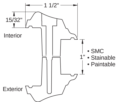
Frame Profile
