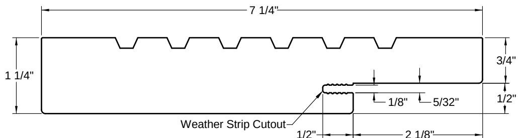
7-1/4" Jamb
