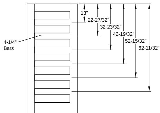
SDL - Flush-Glazed Classic Craft Shaker American - 6'8" Colonial 7 Lite
