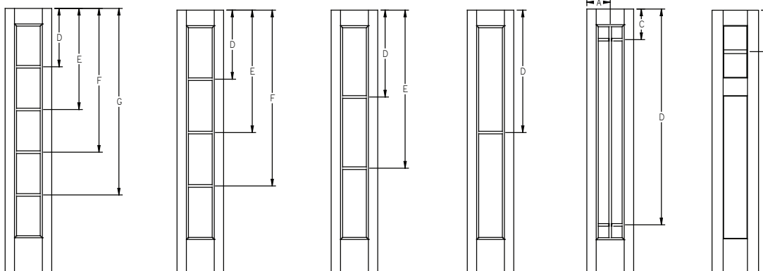
GBG/SDL - Flush-Glazed - Smooth-Star - 6'8" Full Lite Sidelite - 1W5H
