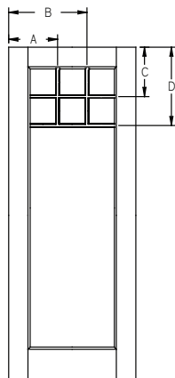
GBG - Flush-Glazed - Smooth-Star - 8'0" Full Lite Craftsman - 3W2H
