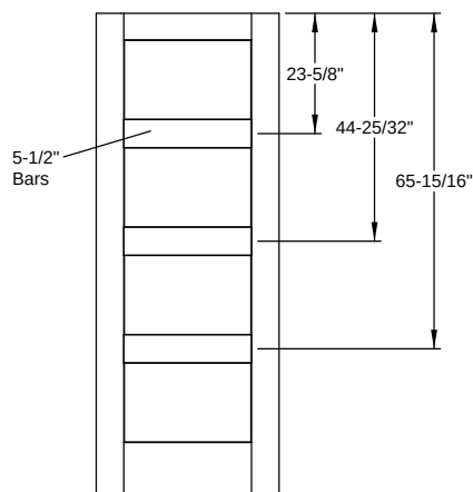
SDL - Flush-Glazed Classic Craft Shaker American - 8'0" Colonial 6 Lite
