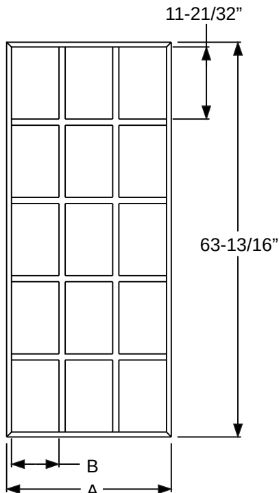
15-Lite
