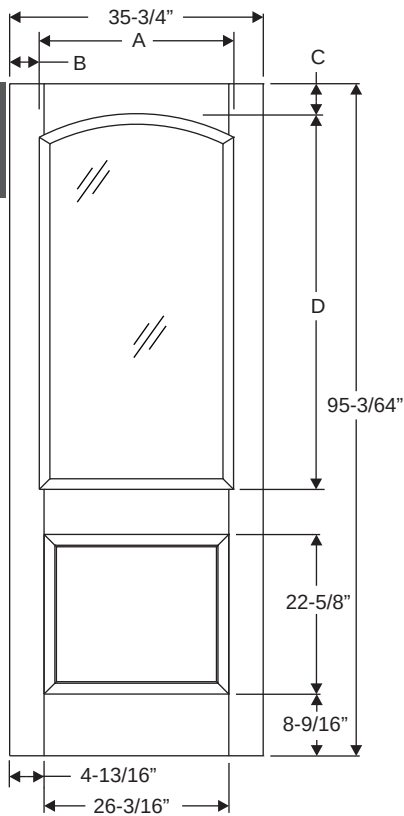
Classic-Craft Panel Dimensions
