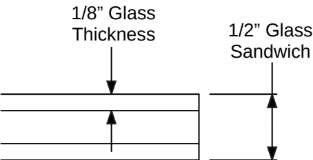
1/2" Glass Sandwich
