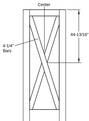
Door Divider - Opaque / SDL - Flush-Glazed Classic Craft Shaker American 8'0" 1 Panel Shaker Double-X 8'0" Full Lite Shaker Double-X
