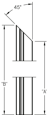
STANDARD BRICKMOULD
