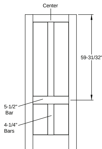
Door Divider - Opaque Classic Craft Shaker American - 8'0" 4 Panel Square Top Shaker
