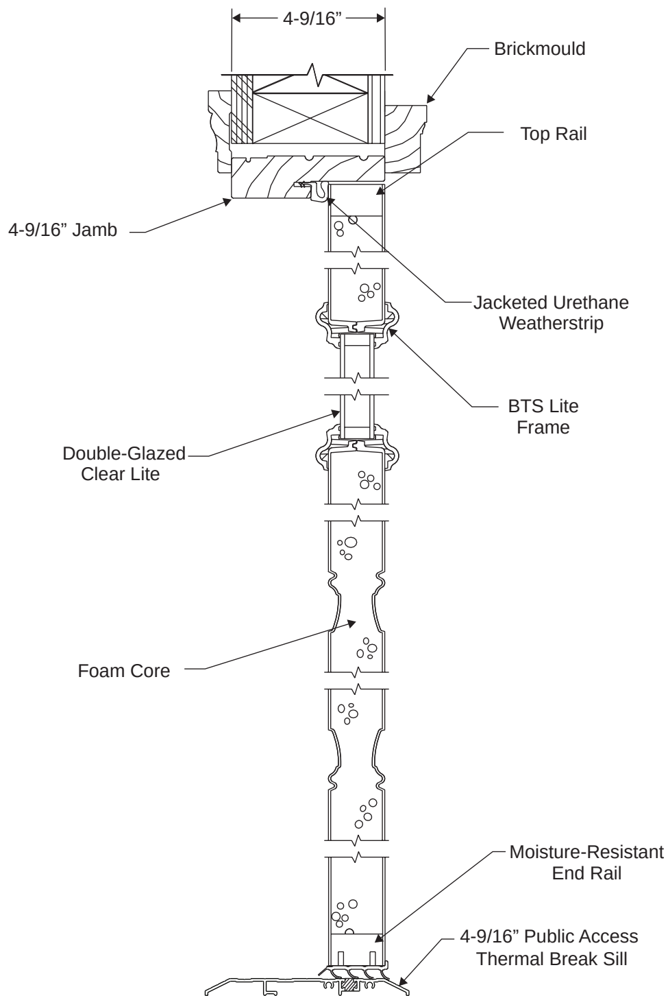
SECTION B-B
