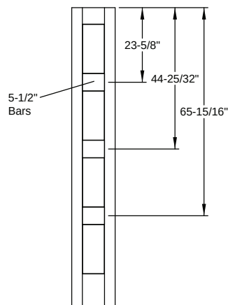
SDL - Flush-Glazed Classic Craft Shaker American - 8'0" Colonial 6 Lite
