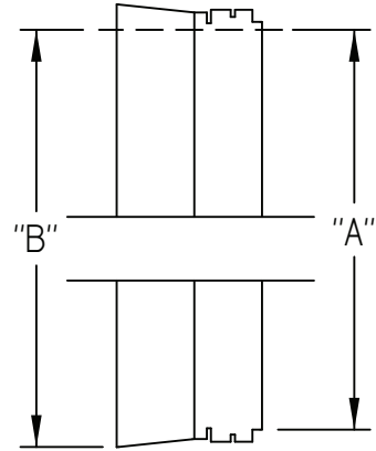
INSWING SILL/SILL GAIN RIGHT RAW CUTDOWN
