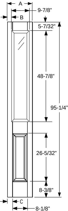
Fiber-Classic/ Smooth-Star/ Steel Panel Dimensions
