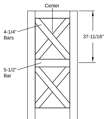
Door Divider - Opaque / SDL - Flush-Glazed Classic Craft Shaker American 6'8" 1 Panel Shaker Double-X 6'8" Full Lite Shaker Double-X
