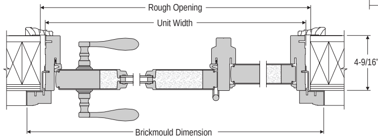
HORIZONTAL SECTION OUTSWING - DOUBLE w/MULLION (LF shown)
