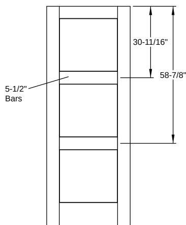
Door Divider - Opaque / SDL - Flush-Glazed Classic Craft Shaker American - 8'0" 5 Panel Shaker - 8'0" Colonial 5 Lite
