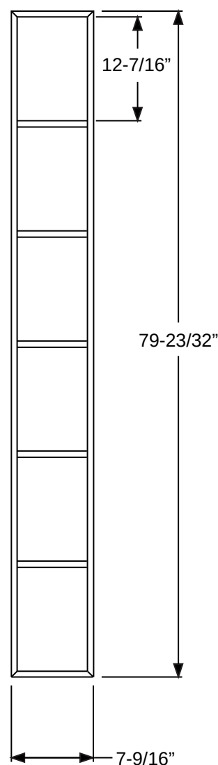
6 Lite FG075L6
