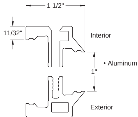
Frame Profile
