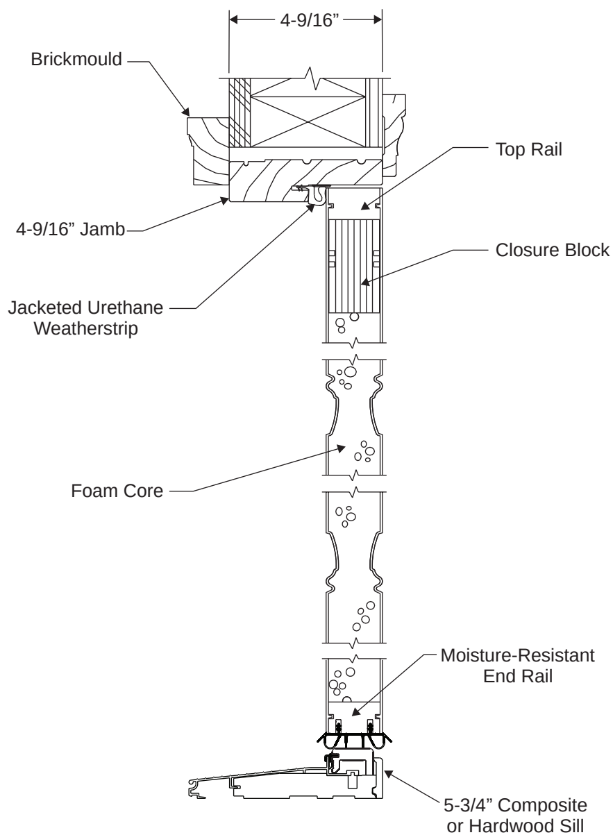
SECTION B-B
