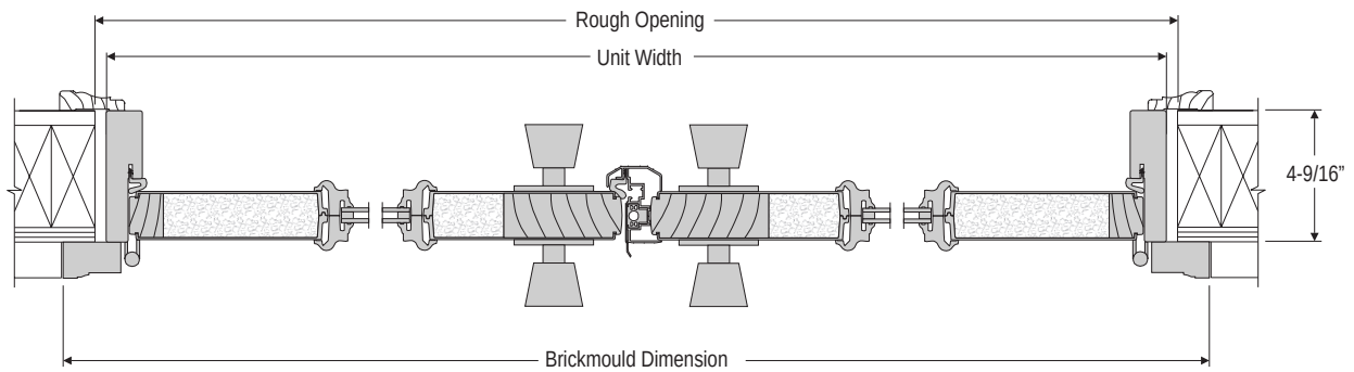
HORIZONTAL SECTION OUTSWING - DOUBLE w/ASTRAGAL (RA shown)
