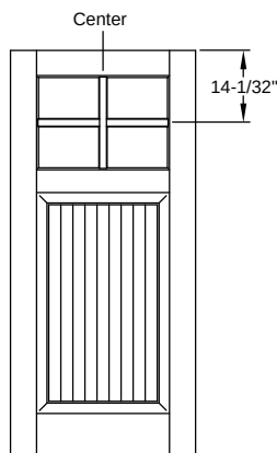
SDL - Flush Glazed Classic Craft Canvas & Icon - 6'8" Craftsman 4 Lite 2W2H
