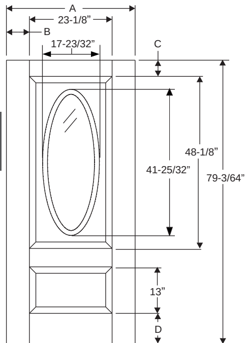
Fiber-Classic/ Smooth-Star/ Steel Panel Dimensions
