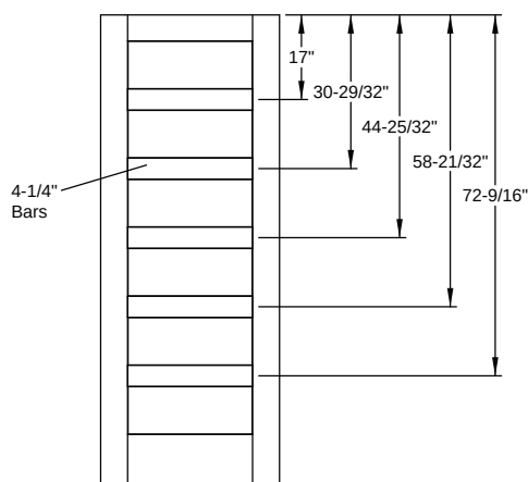
SDL - Flush-Glazed Classic Craft Shaker American - 8'0" Colonial 8 Lite
