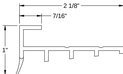
Inactive Panel Door Bottom - Composite Outswing Sill
