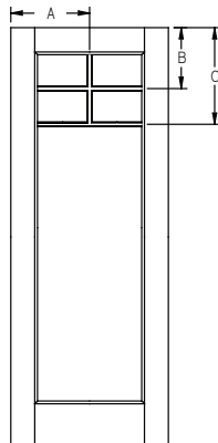
GBG - Flush-Glazed - Smooth-Star - 8'0" Full Lite Craftsman - 2W2H
