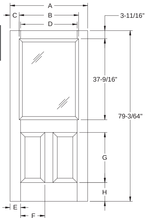
Classic-Craft Panel Dimensions
