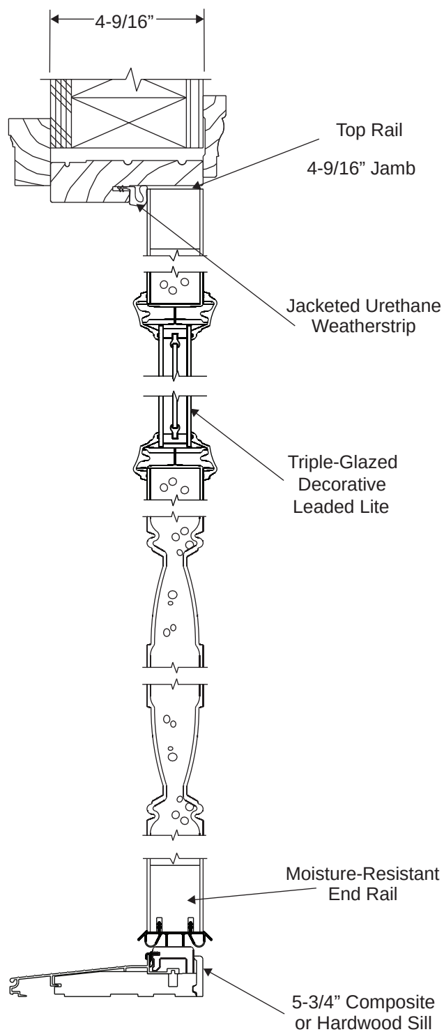
SECTION B-B
