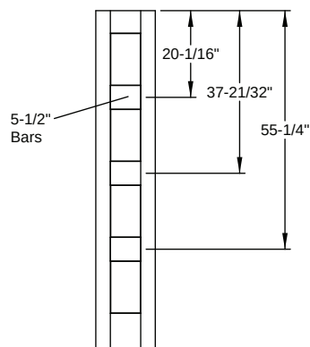
SDL - Flush-Glazed Classic Craft Shaker American - 6'8" Colonial 4 Lite
