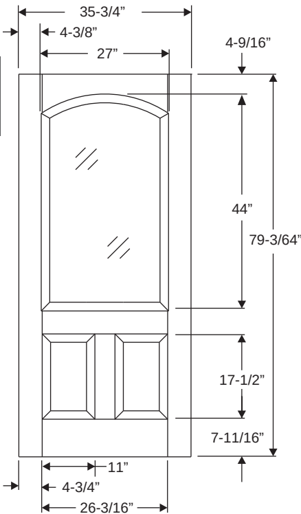
Classic-Craft Panel Dimensions
