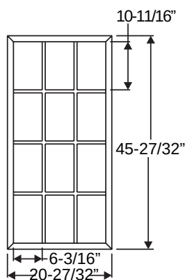
12-Lite (2247)
