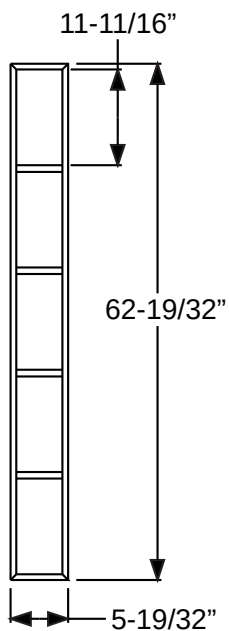
5-Lite Sidelite (0764)
