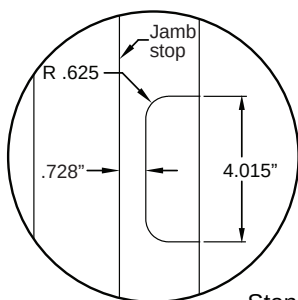
Standard Hinge
