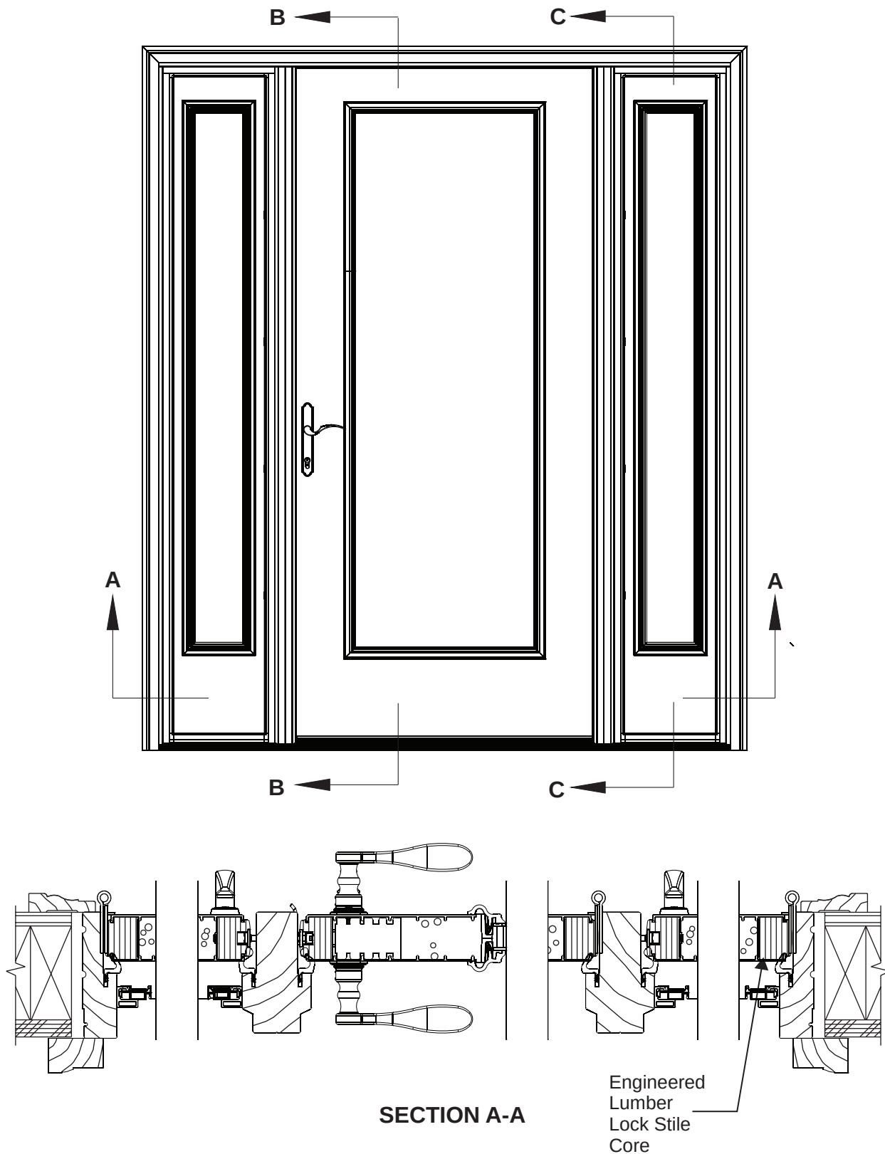
6/8 Door with Vented Sidelites, Continuous Frame, with Casing
