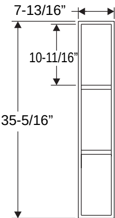
3-Lite CPG743L3
