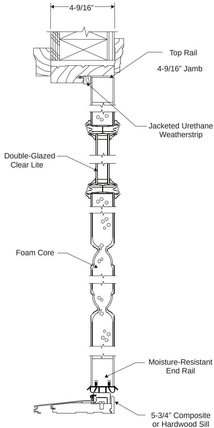
SECTION B-B
