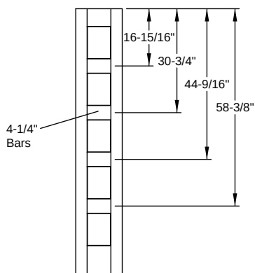
SDL - Flush-Glazed Classic Craft Shaker American - 6'8" Colonial 5 Lite
