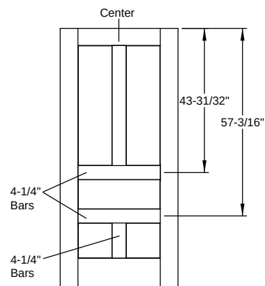
Door Divider - Opaque Classic Craft Shaker American - 6'8" 5 Panel Square Top Shaker
