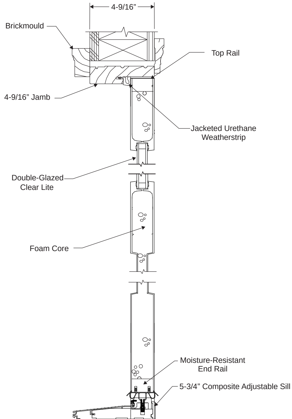
SECTION B-B
