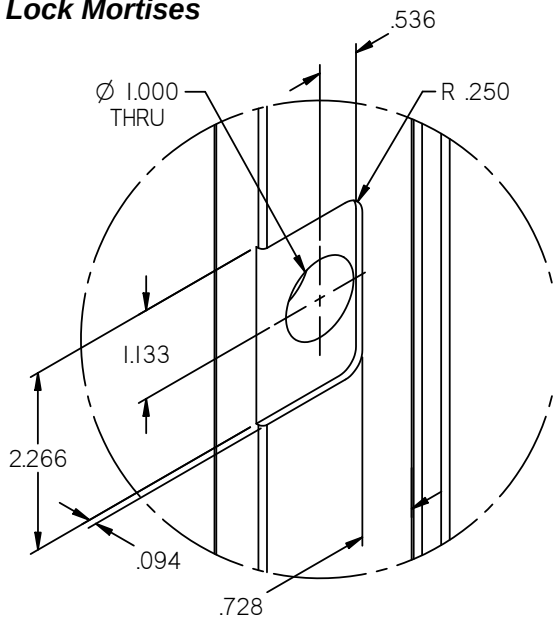
LATCH MACHINING
