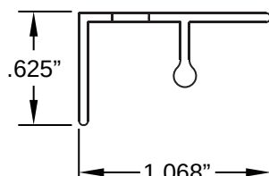
Screen Track
