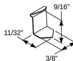
Retaining Clip
