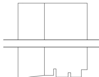
Composite/Hardwood Inswing Adjustable Sill (Entry Mullion Shown)
