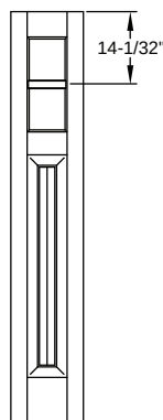
SDL - Flush Glazed Classic Craft Canvas & Icon - 6'8" Craftsman Sidelite 2 Lite 1W2H
