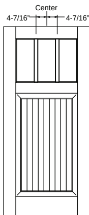
SDL - Flush Glazed Classic Craft Canvas & Icon - 6'8" Craftsman 3 Lite 3W1H
