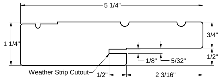
5-1/4" Jambs
