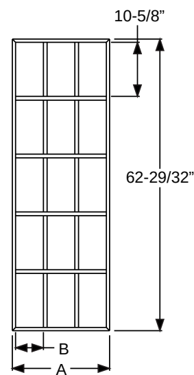
15-Lite (2264)
