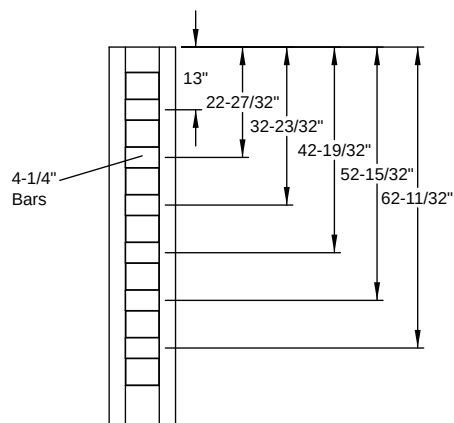
SDL - Flush-Glazed Classic Craft Shaker American - 6'8" Colonial 7 Lite
