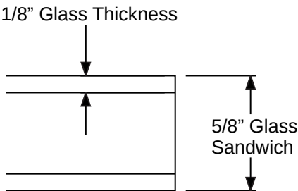
5/8" Glass Sandwich
