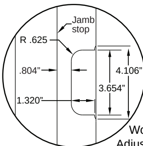
Standard Hinge
