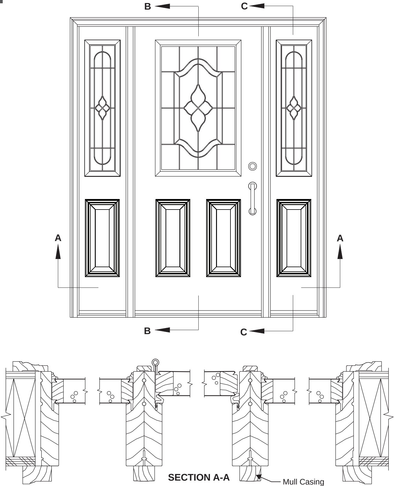
6/8 Door/Sidelites with Separate Frames, Joined, with Casing
