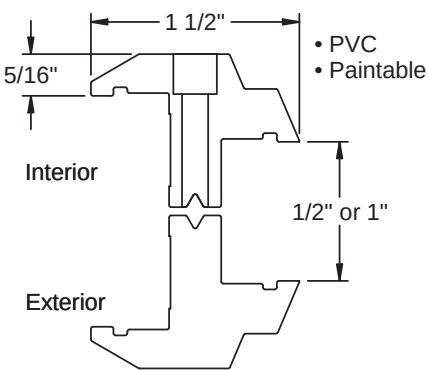
Frame Profile
