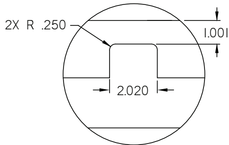
STANDARD MULLION
