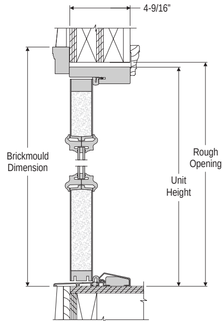
VERTICAL SECTION OUTSWING THERMAL BREAK
