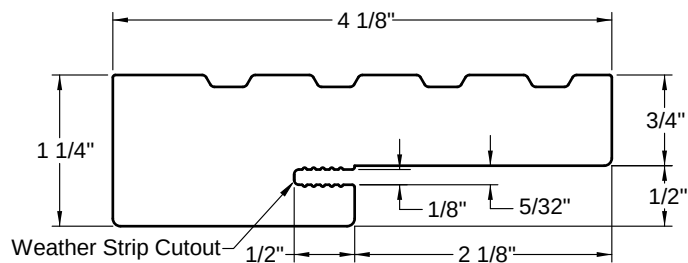
4-1/8" Jamb
