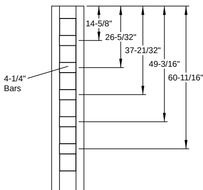
SDL - Flush-Glazed Classic Craft Shaker American - 6'8" Colonial 6 Lite
