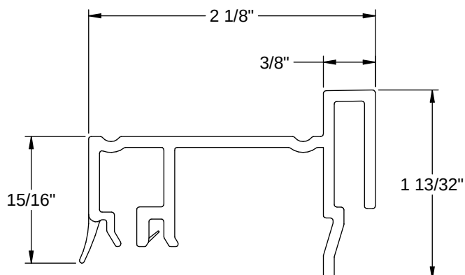
Inswing Sidelite Seat for U1 Door Slabs
