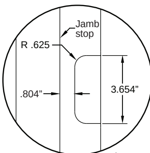
Therma-Tru Composite Jamb Adjustable Hinge
