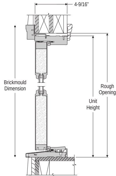
VERTICAL SECTION OUTSWING
