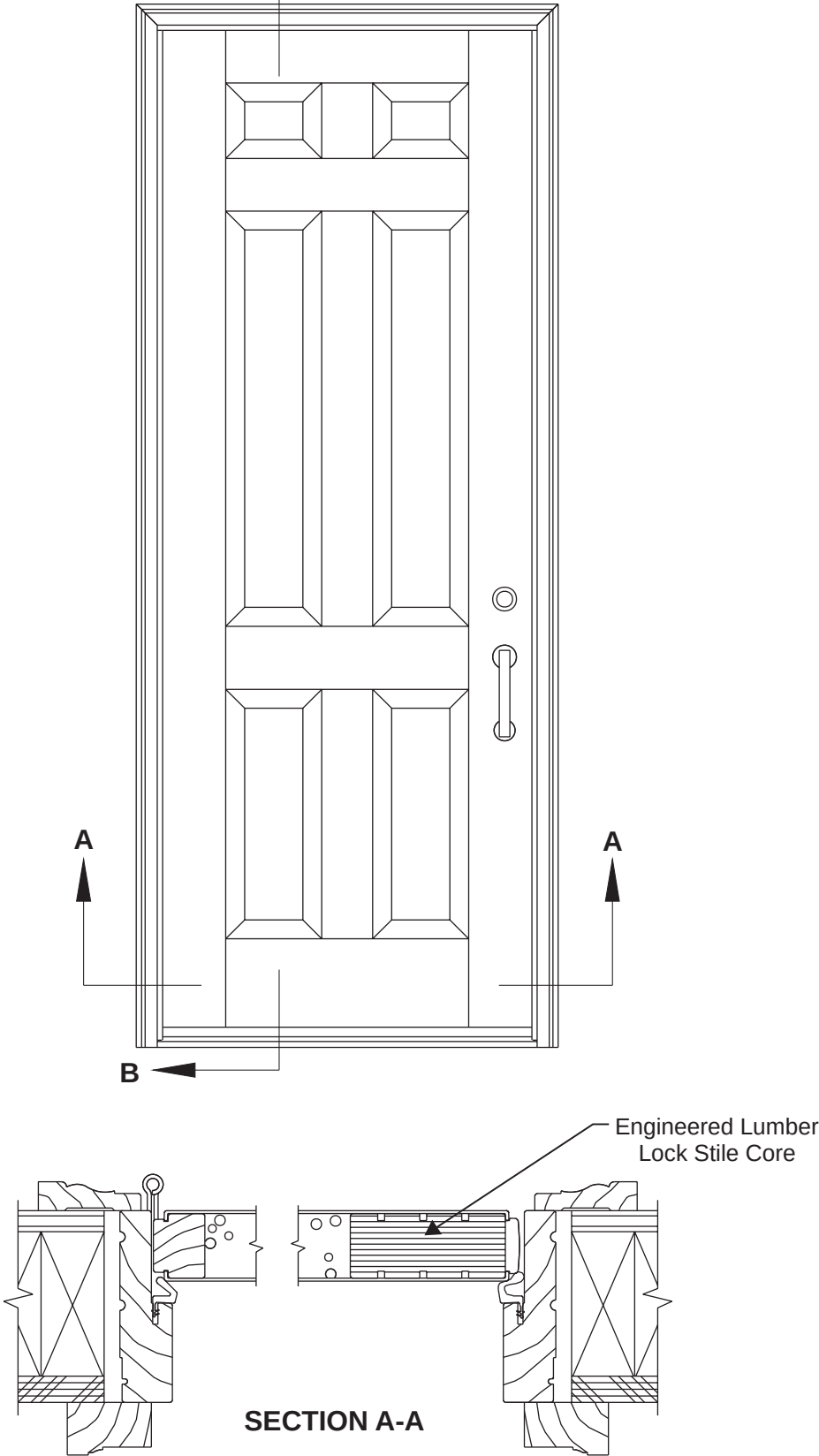
8/0 Single Door, Inswing B
