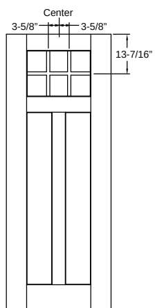
SDL - Flush-Glazed - Smooth-Star - 8'0" Craftsman Lite 2 Panel Shaker - 3W2H
