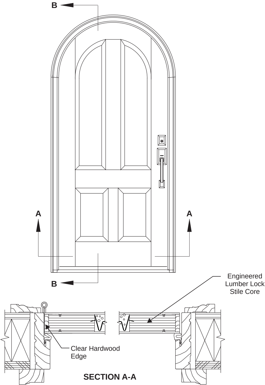
6/8 Single Radius Top Door, Inswing
