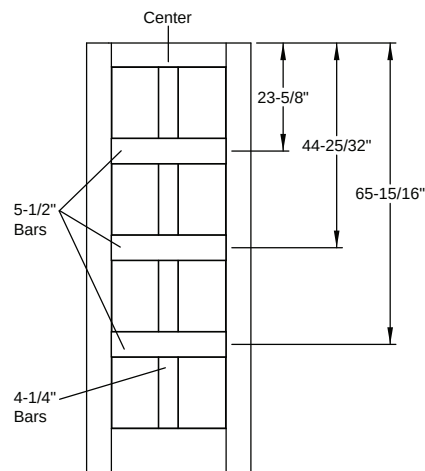
SDL - Flush-Glazed Classic Craft Shaker American - 8'0" Colonial 8 Lite
