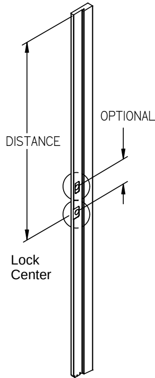
Spread Mullion
