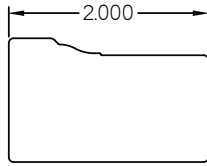
STANDARD BRICKMOULD
