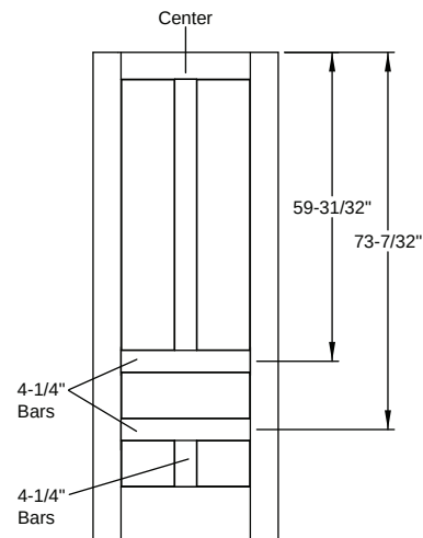
Door Divider - Opaque Classic Craft Shaker American - 8'0" 5 Panel Square Top Shaker
