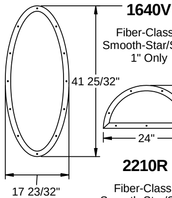
Frame Profile
