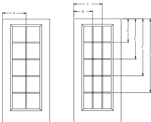
GBG/SDL - Lip Lite - 6'8" Full Lite - 3W5H and 2W5H
