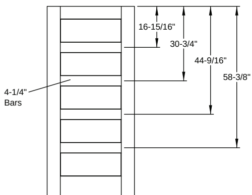
Door Divider - Opaque / SDL - Flush-Glazed Classic Craft Shaker American - 6'8" 5 Panel Shaker - 6'8" Colonial 5 Lite
