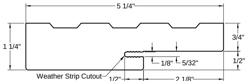
5-1/4" Jamb
