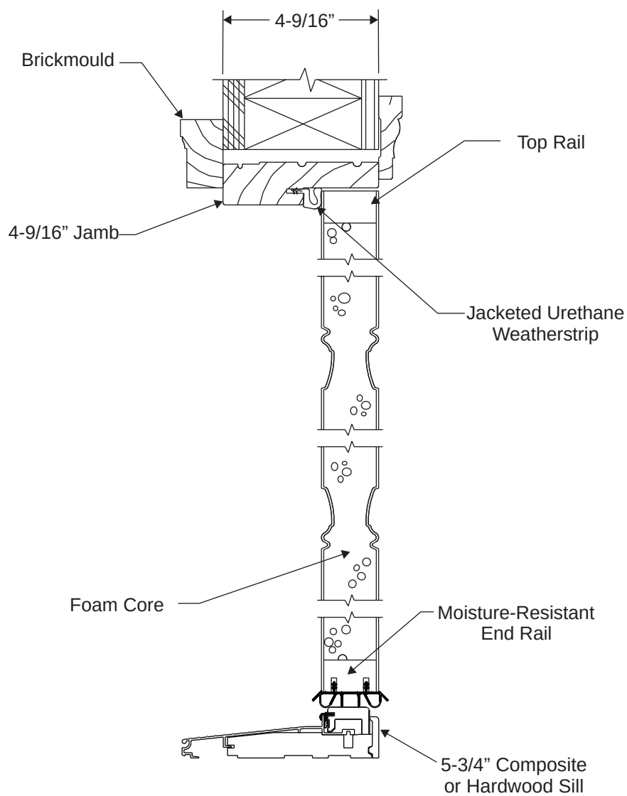
SECTION B-B
