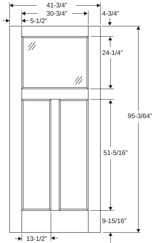
8' Craftsman Expanded Lite 2 Panel Flush-Glazed
