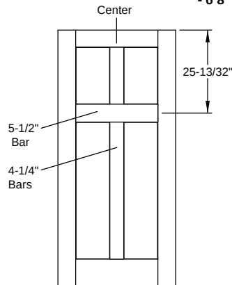
Door Divider - Opaque / SDL - Flush Glazed Classic Craft Shaker American - 6'8" 4 Panel Craftsman Shaker - 6'8" Craftsman 4 Lite
