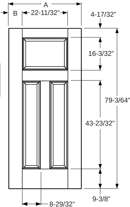
Fiber-Classic/ Smooth-Star/ Steel Panel Dimensions
