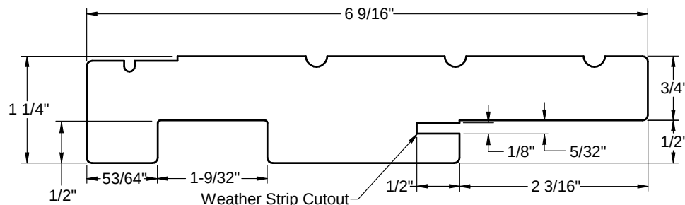
6-9/16" Patio Jambs (for sliding screens)
