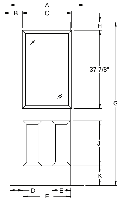
Fiber-Classic/ Smooth-Star/ Steel Panel Dimensions
