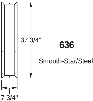
Frame Profile
