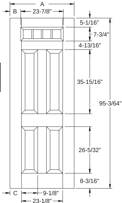
Fiber-Classic/ Smooth-Star/ Steel Panel Dimensions
