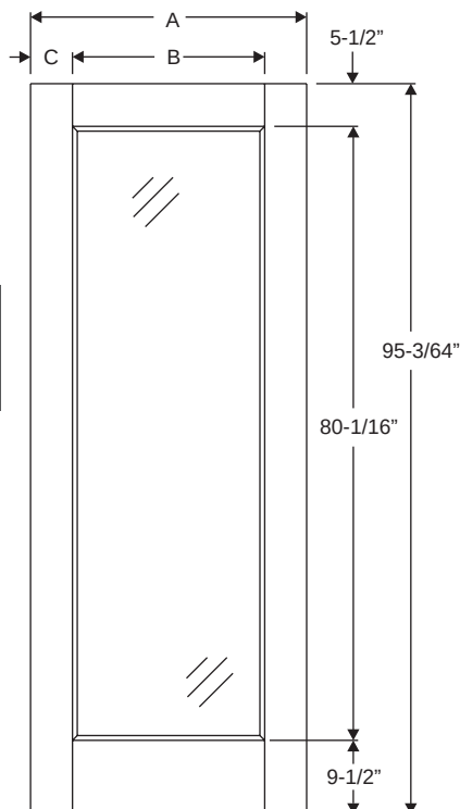
Fiber-Classic/ Smooth-Star/ Steel Panel Dimensions
