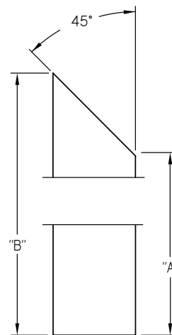
MITER FLAT CASING
