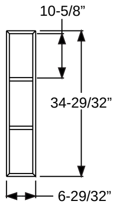
3-Lite Sidelite (0836)
