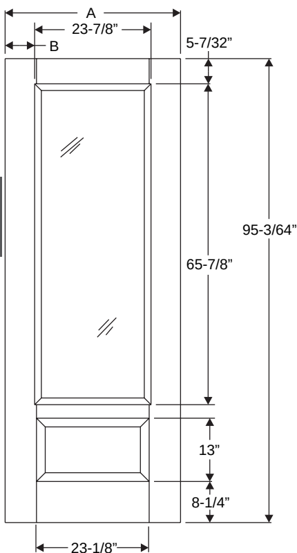
Fiber-Classic/ Smooth-Star/ Steel Panel Dimensions
