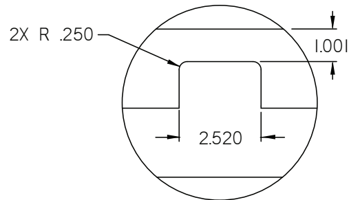
WIDE MULLION
