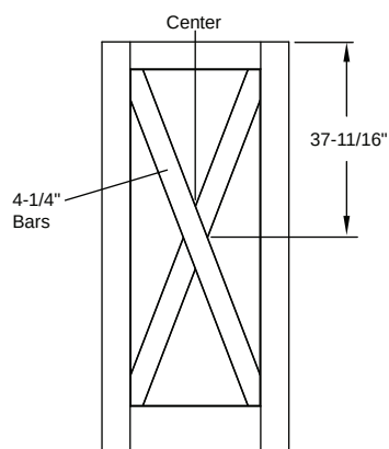
Door Divider - Opaque / SDL - Flush-Glazed Classic Craft Shaker American 6'8" 1 Panel Shaker X-Brace 6'8" Full Lite Shaker X-Brace
