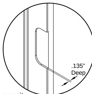
Therma-Tru Composite Jamb Adjustable Hinge
