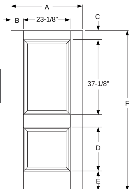
Fiber-Classic/ Smooth-Star/ Steel Panel Dimensions
