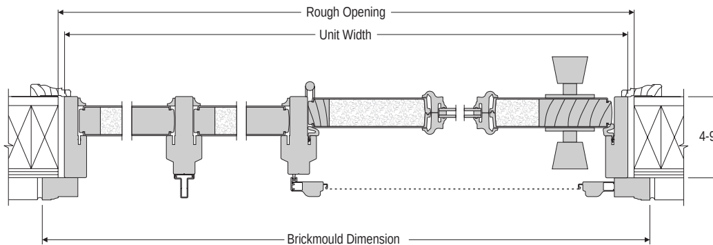
HORIZONTAL SECTION INSWING - TRIPLE (FFL shown)
