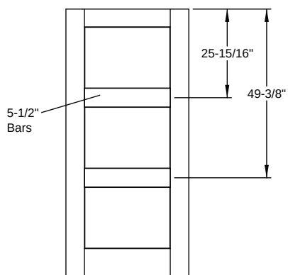
Door Divider - Opaque / SDL - Flush-Glazed Classic Craft Shaker American - 6'8" 3 Panel Shaker - 6'8" Colonial 3 Lite
