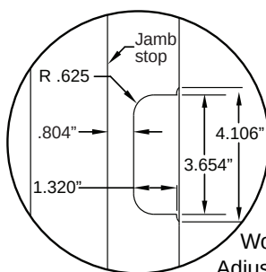
Standard Hinge
