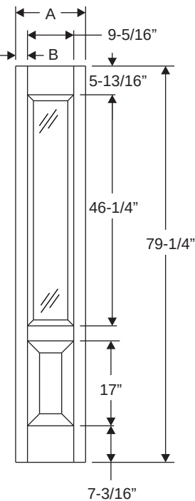
Classic-Craft Panel Dimensions
