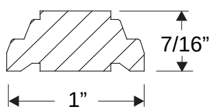
Wood Grille Section (Flush-Glazed)
