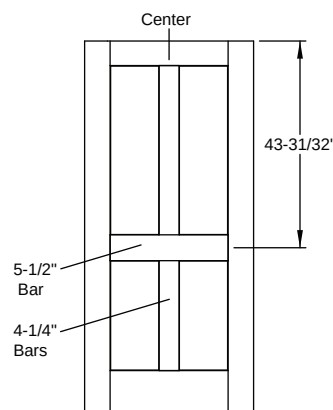
Door Divider - Opaque Classic Craft Shaker American - 6'8" 4 Panel Square Top Shaker
