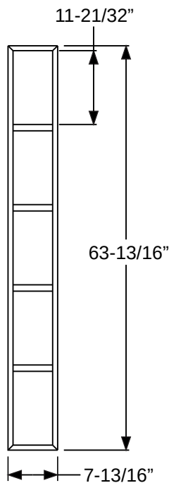
5-Lite PG0864L5
