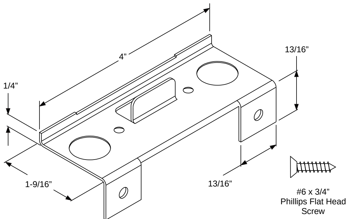
Fiber-Class, Smooth-Star and Steel Door Units Part # MS00TPC
