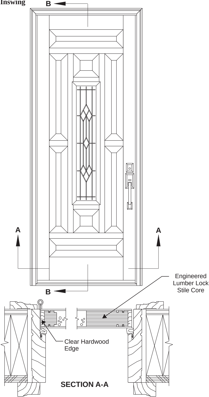
8/0 Single Door, Inswing
