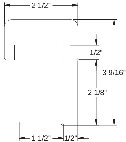
Composite Standard & Wide Mullion
