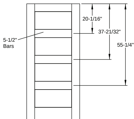
Door Divider - Opaque / SDL - Flush-Glazed Classic Craft Shaker American - 6'8" 4 Panel Shaker - 6'8" Colonial 4 Lite
