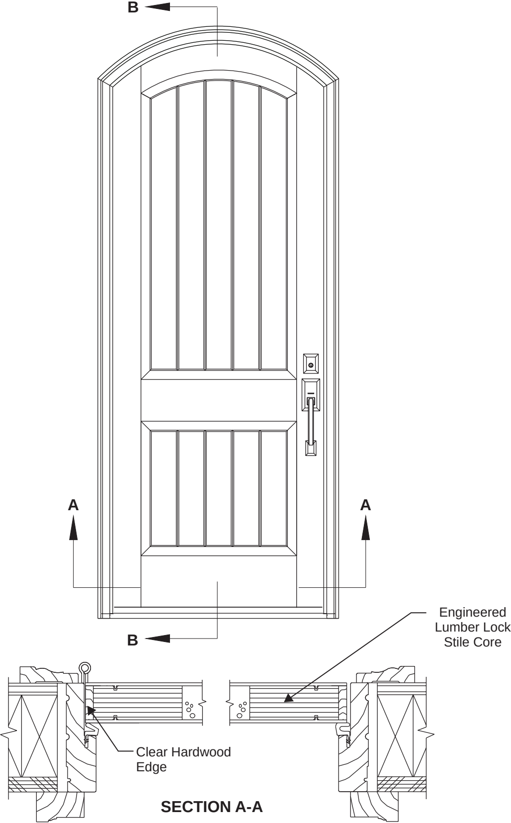
8/0 Single Arch Top Door, Inswing
