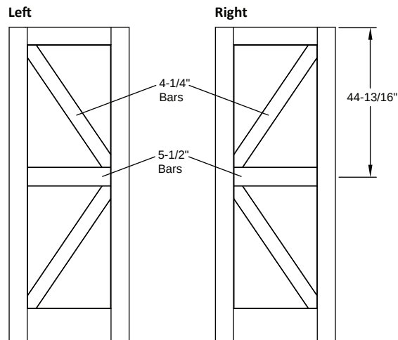
Door Divider - Opaque / SDL - Flush-Glazed Classic Craft Shaker American 8'0" 1 Panel Shaker Double-Z 8'0" Full Lite Shaker Double-Z
