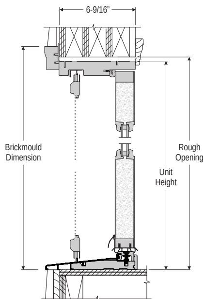
VERTICAL SECTION INSWING - 6-9/16" w/STANDARD SCREEN
