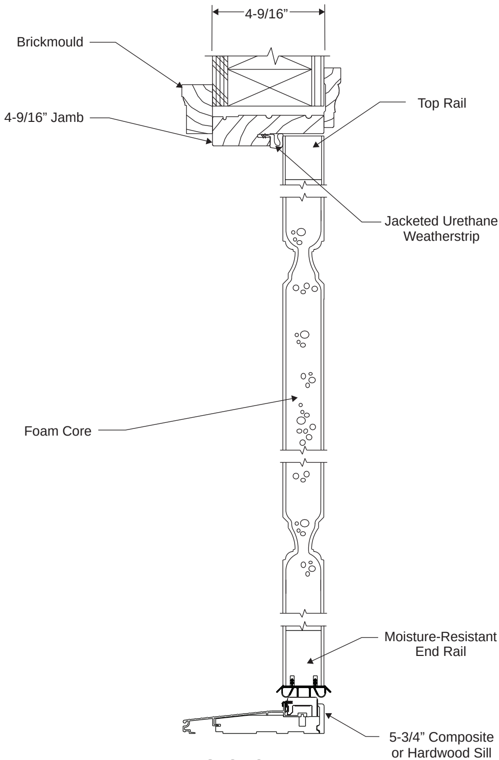
SECTION B-B
