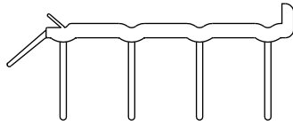
Sweep/Replacement Door Bottom DB30SWP
