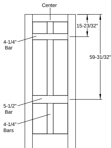
Door Divider - Opaque Classic Craft Shaker American - 8'0" 6 Panel Shaker
