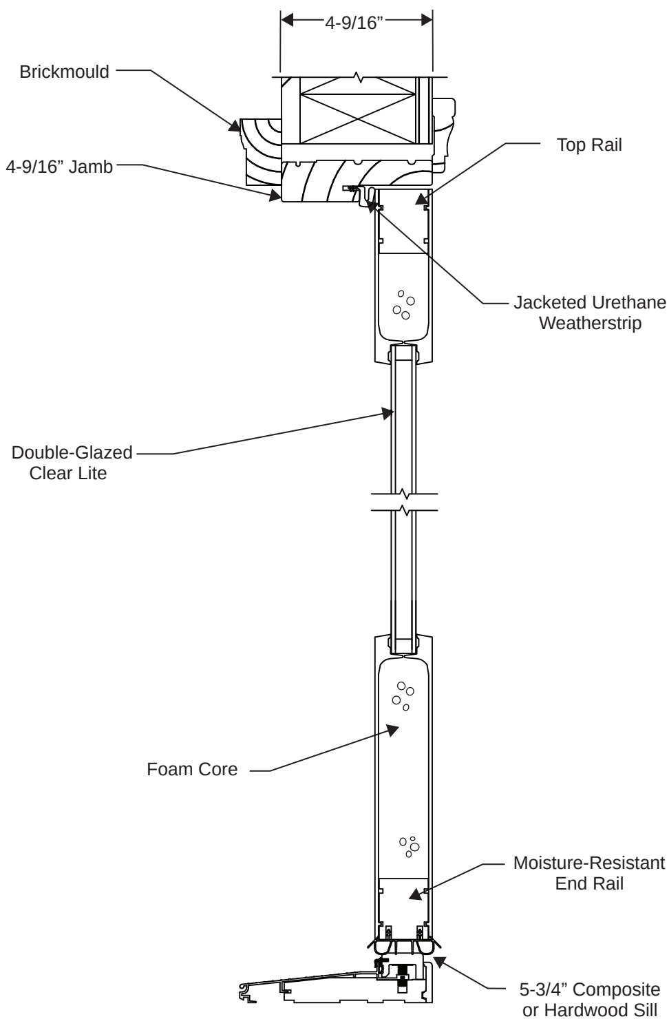
SECTION B-B
