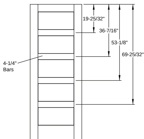
SDL - Flush-Glazed Classic Craft Shaker American - 8'0" Colonial 7 Lite
