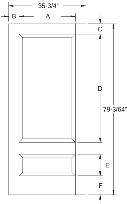
Classic-Craft Panel Dimensions
