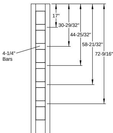
SDL - Flush-Glazed Classic Craft Shaker American - 8'0" Colonial 6 Lite
