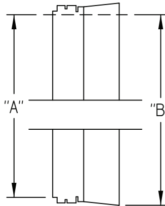
INSWING SILL/SILL GAIN LEFT RAW CUTDOWN
