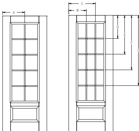
GBG/SDL - Lip Lite - 8'0" 3/4 Lite - 3W5H and 2W5H
