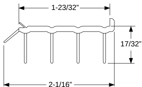
Sweep/Replacement Door Bottom
