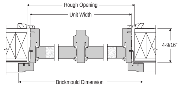
HORIZONTAL SECTION OUTSWING - FIXED/FIXED
