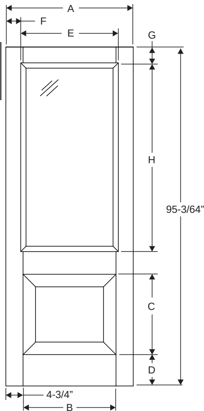
Classic-Craft Panel Dimensions
