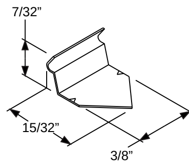
Retaining Clip
