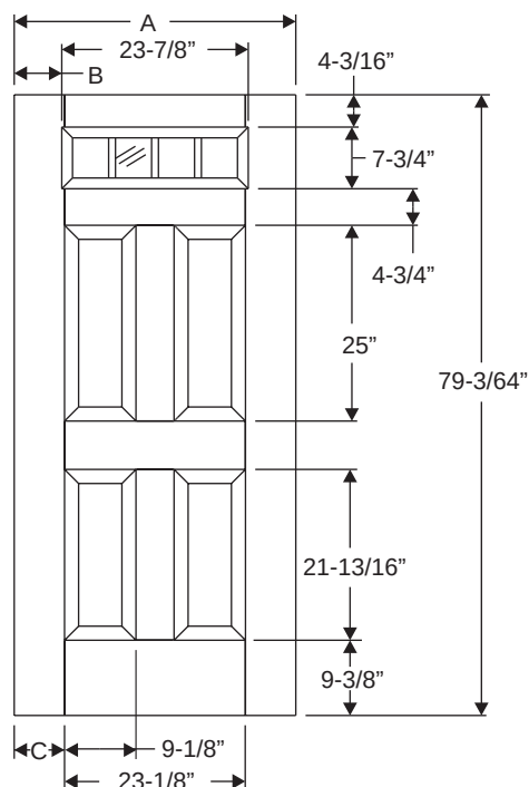
Fiber-Classic/ Smooth-Star/ Steel Panel Dimensions
