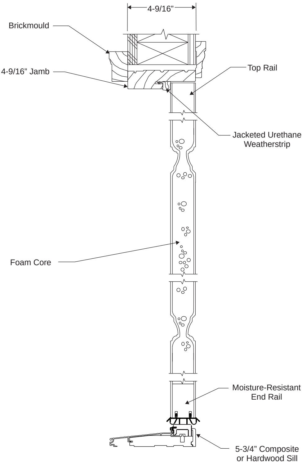
SECTION B-B
