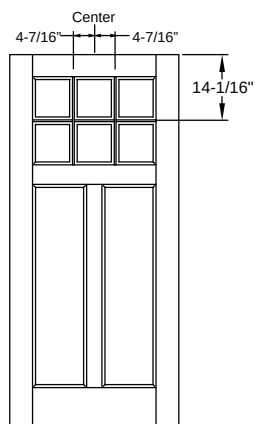
SDL - Flush Glazed Classic Craft American - 6'8" Craftsman 6 Lite 3W2H
