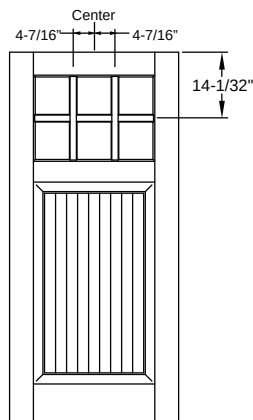
SDL - Flush Glazed Classic Craft Canvas & Icon - 6'8" Craftsman 6 Lite 3W2H
