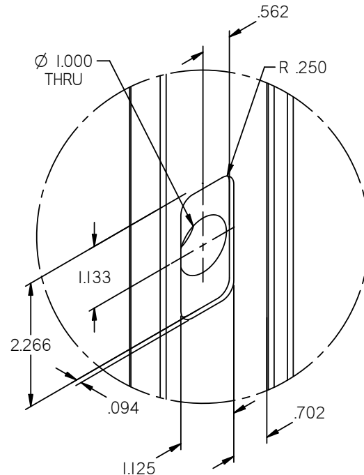
OPTIONAL DEADBOLT MACHINING
