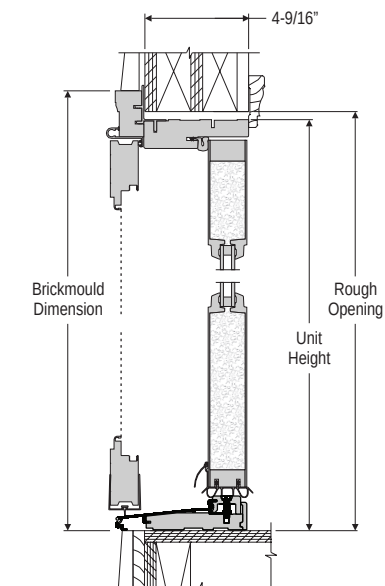
VERTICAL SECTION INSWING - DOUBLE w/ASTRAGAL w/HINGED SCREEN
