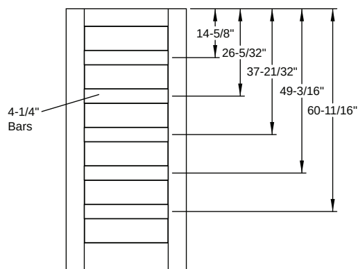
SDL - Flush-Glazed Classic Craft Shaker American - 6'8" Colonial 6 Lite
