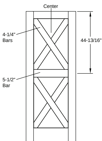
Door Divider - Opaque / SDL - Flush-Glazed Classic Craft Shaker American 8'0" 1 Panel Shaker Bottom-X 8'0" Full Lite Shaker Bottom-X
