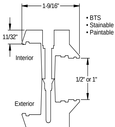
Frame Profile
