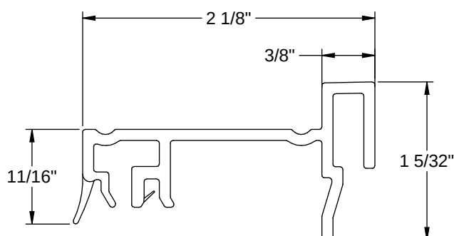
Inswing Sidelite Seat for Standard Sidelite Slabs
