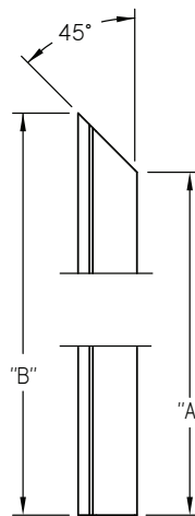
FLORIDA BRICKMOULD
