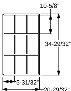
9-Lite (2236)
