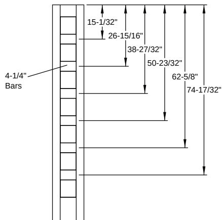
SDL - Flush-Glazed Classic Craft Shaker American - 8'0" Colonial 7 Lite
