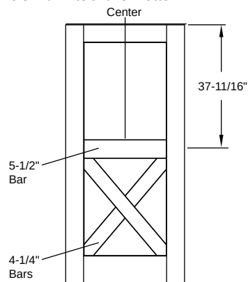
Door Divider - Opaque / SDL - Flush-Glazed Classic Craft Shaker American 6'8" 1 Panel Shaker Bottom-X 6'8" Full Lite Shaker Bottom-X
