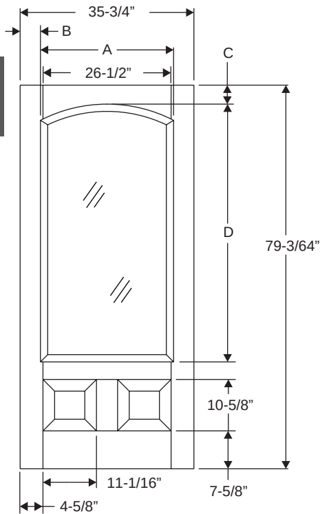
Classic-Craft Panel Dimensions
