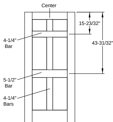
Door Divider - Opaque Classic Craft Shaker American - 6'8" 6 Panel Shaker
