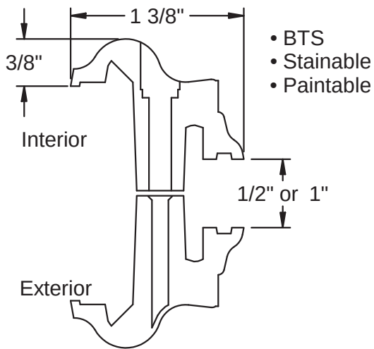
Frame Profile
