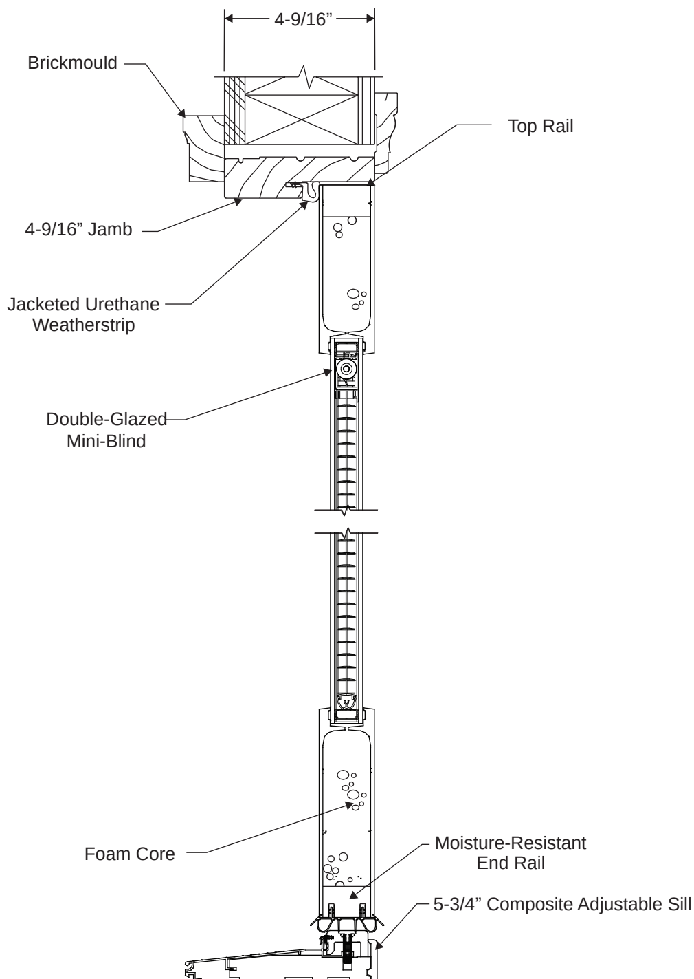
SECTION B-B
